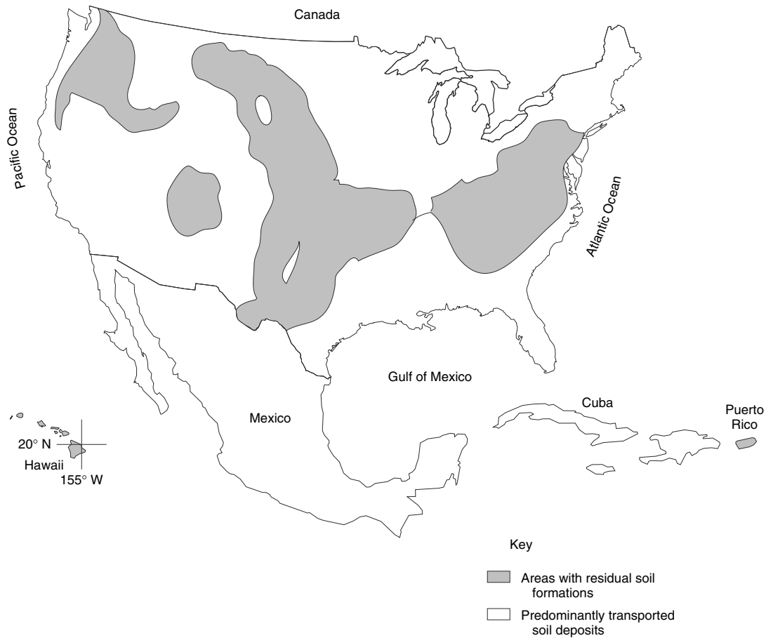
Figure 4 Distribution of transported soil and residual soil formations for the United States. (Compiled from several sources)
